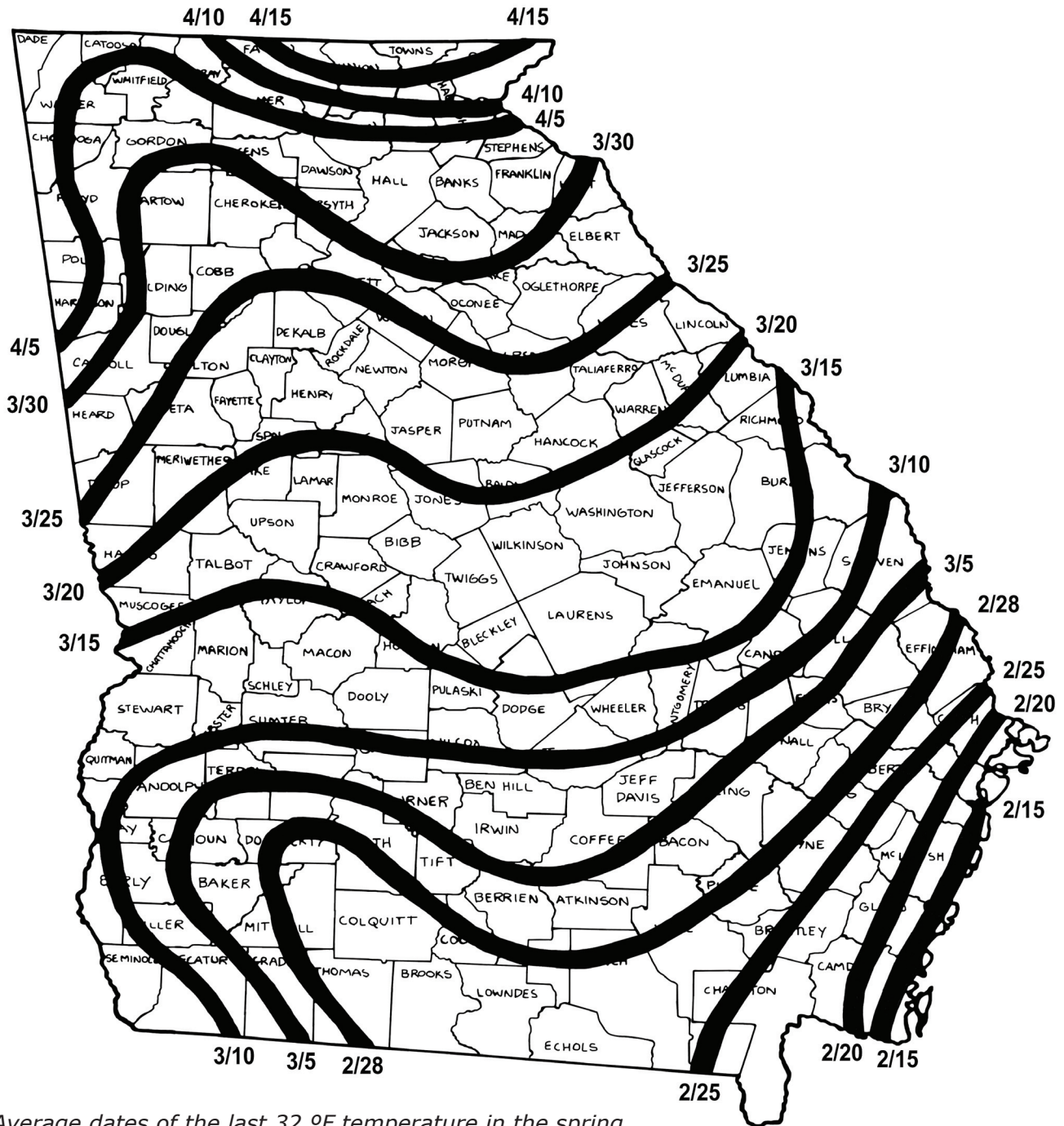
Average dates of the last 32 °F temperature in the spring.
