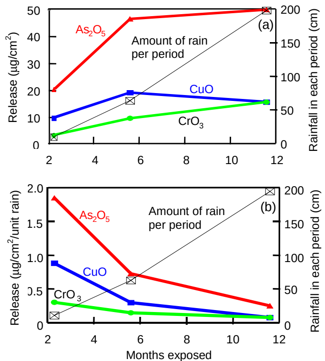
Figure I-4—Release of copper, chromium, and arsenic into rainwater collected from CCA-C-treated decking. Rate of release expressed as (a) µg/cm² and (b) µg/cm²/unit rain. 1 unit = 2.54 cm (1 in.).
