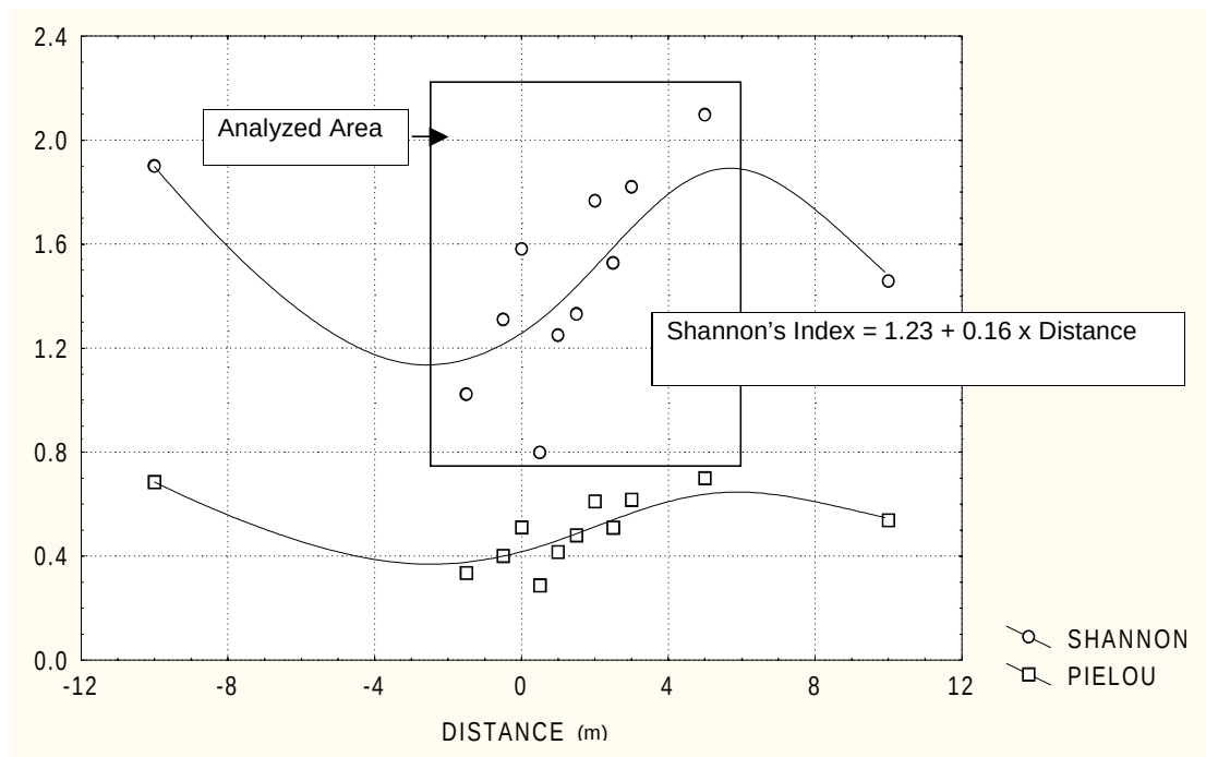
Figure II-20—Shannon's and Pielou's indices for infauna data collected at ACQ-B site on day +336. Area subjected to regression analysis is blocked; resulting significant regression is given.
