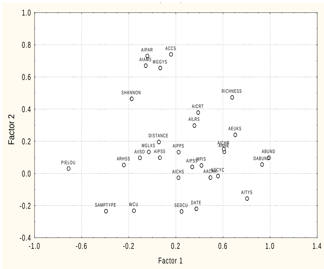
Figure II-21—Results of factor analysis on all invertebrate data collected at ACQ-B site. Principal factors (MINRES) extraction followed by Varimax normalization. See Appendix for designation of variables.
