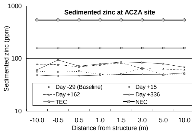
Figure II–25—Sediment concentrations of zinc at ACZA site as function of time and distance from structure located at 0 m. TEC and high NEC (Jones and others 1997) provided for reference.
