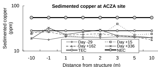
Figure II–24—Sediment concentrations of copper at ACZA site as function of time and distance from structure located at 0 m. TEC and high NEC (Jones and others 1997) provided for reference.
