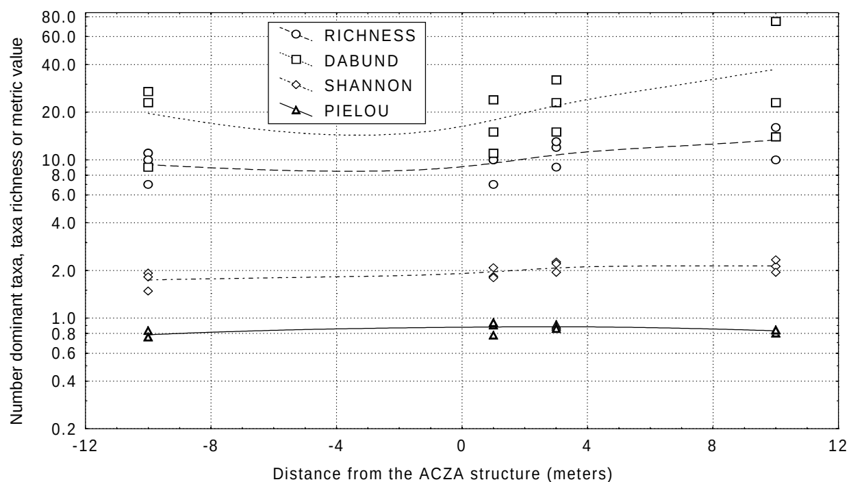
Figure II-26—Total taxa richness, dominant taxa abundance, and Shannon’s and Pielou’s indices for invertebrates collected from artificial substrates at ACZA site on day +15. Distance-weighted least-squares regression lines are provided for each endpoint.
