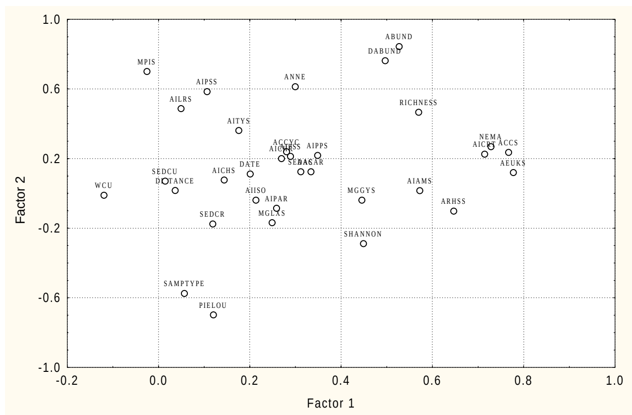
Figure II-40—Results of factor analysis on all invertebrate data collected at ACZA site. MINRES extraction followed by Varimax normalization.
