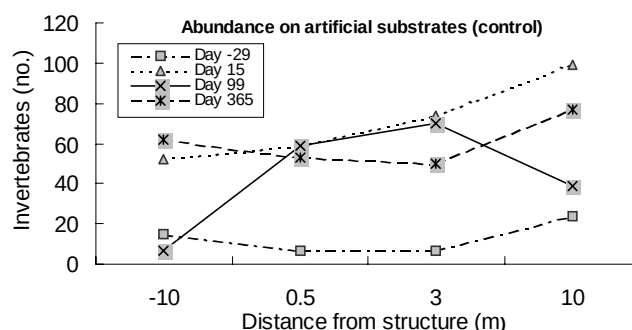
Figure II-8—Total abundance of infauna collected on 10-plate Hester-Dendy artificial substrate collectors at mechanical control site.
