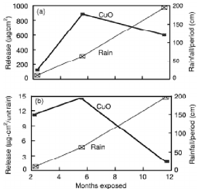
Figure I-7—Release of copper into rainwater collected from ACQB-treated decking. Rate of release expressed as (a) µg/cm² and (b) µg·cm²/unit rain. 1 unit = 22.54 cm (1 in.).
