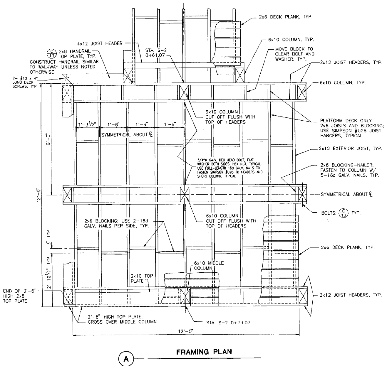
Figure I-10—Framing details for construction of ACQ-B viewing platform, top view.
