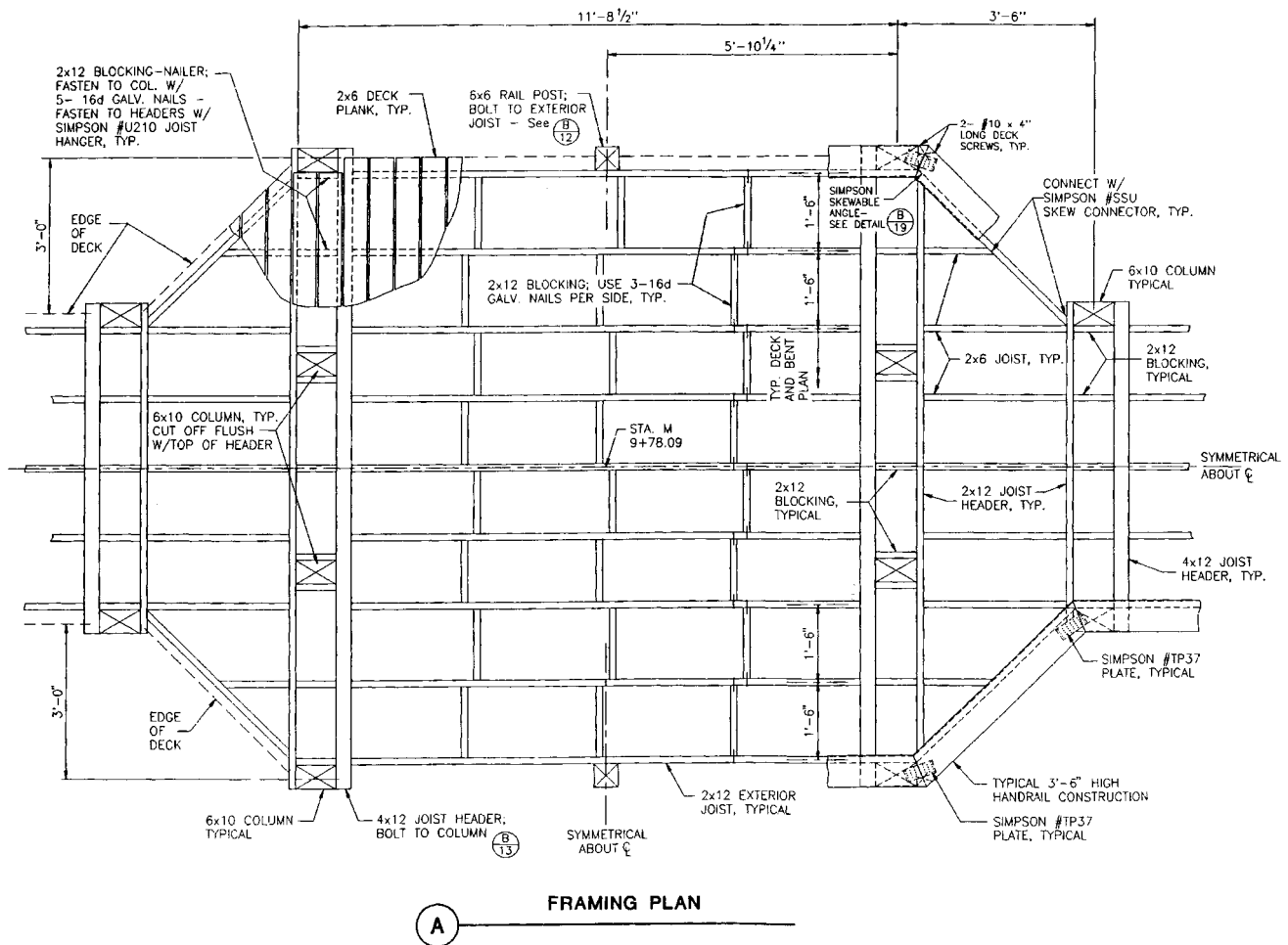
Figure I-12—Framing details for construction of CCA-C viewing platform, top view.
