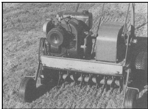
Figure 11. Vertical mower.
